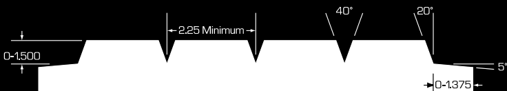
Notching Pattern for Standard Duct Notchers
